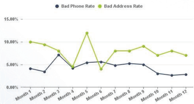
Data Quality
